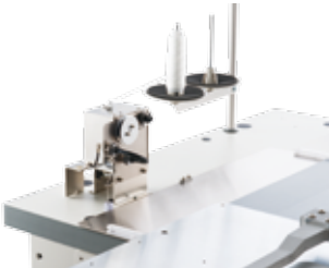
Constant-quantity bobbin thread feeding mechanism
