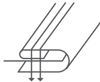
Right Angle Bias Binder-A Type
