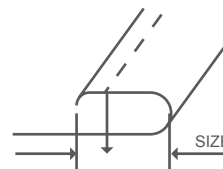
Single Upturn Hemmer
